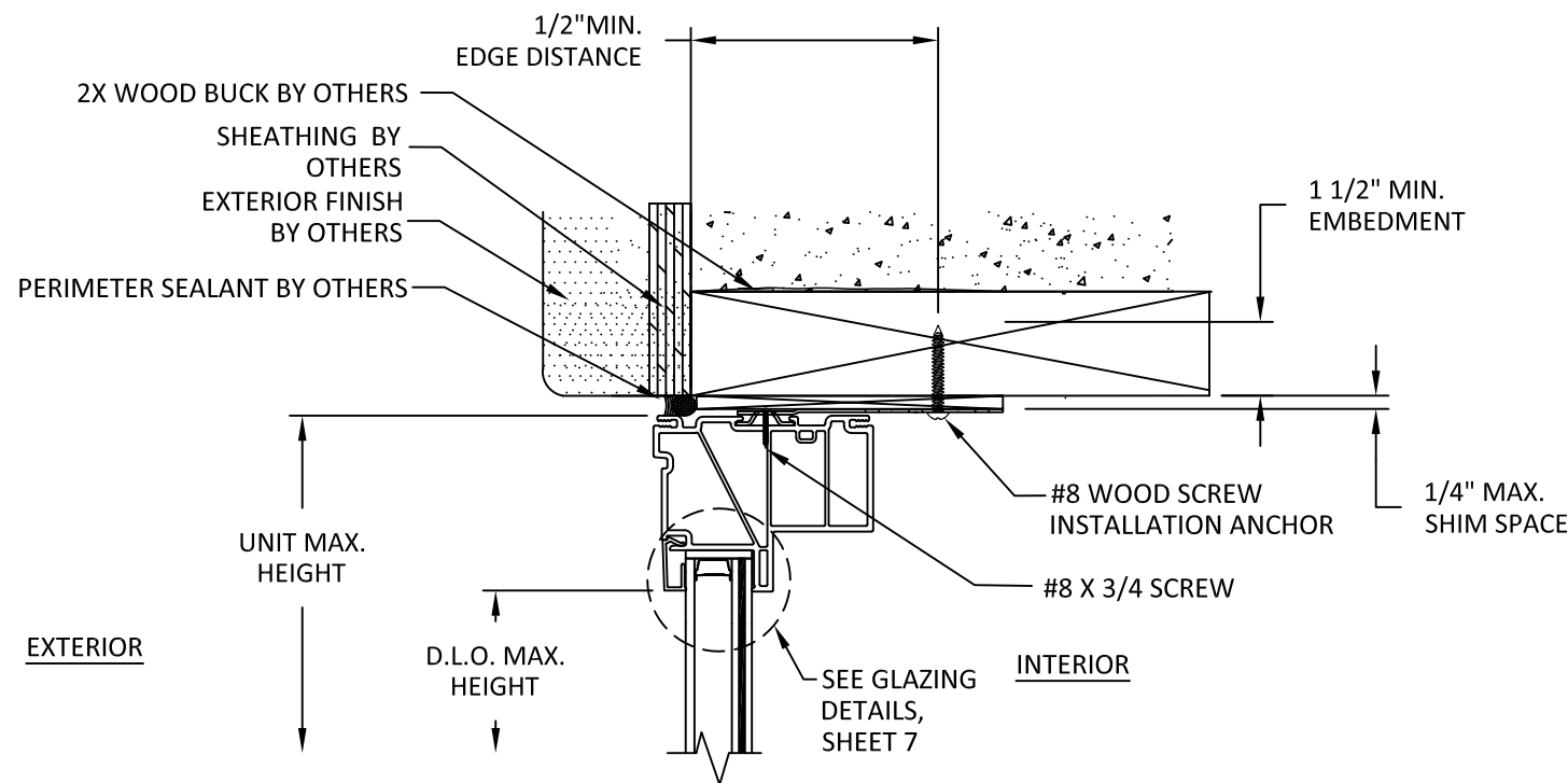
A 6 VERTICAL SECTION
